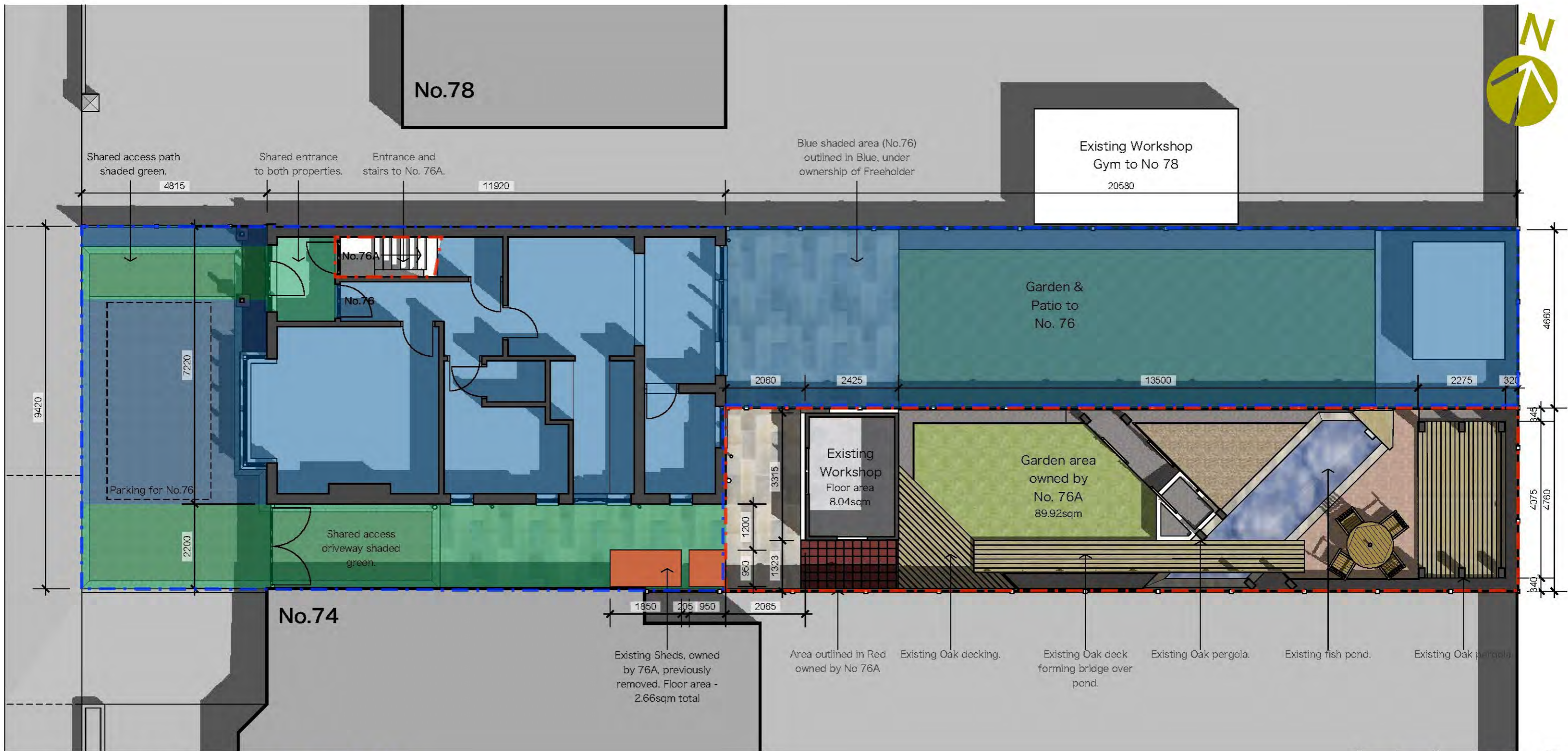
Ground Floor Layout as existing
